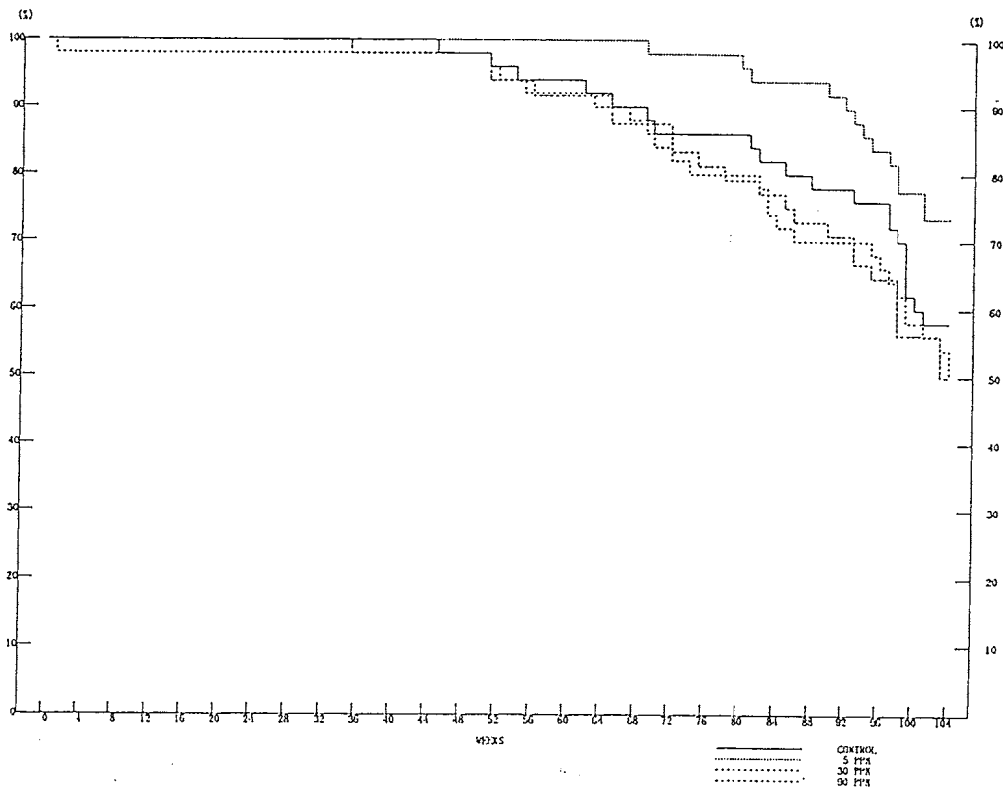
FIGURE 9 SURVIVAL ANIMAL RATE : MOUSE:FEMALE (TWO-YEAR STUDY)
