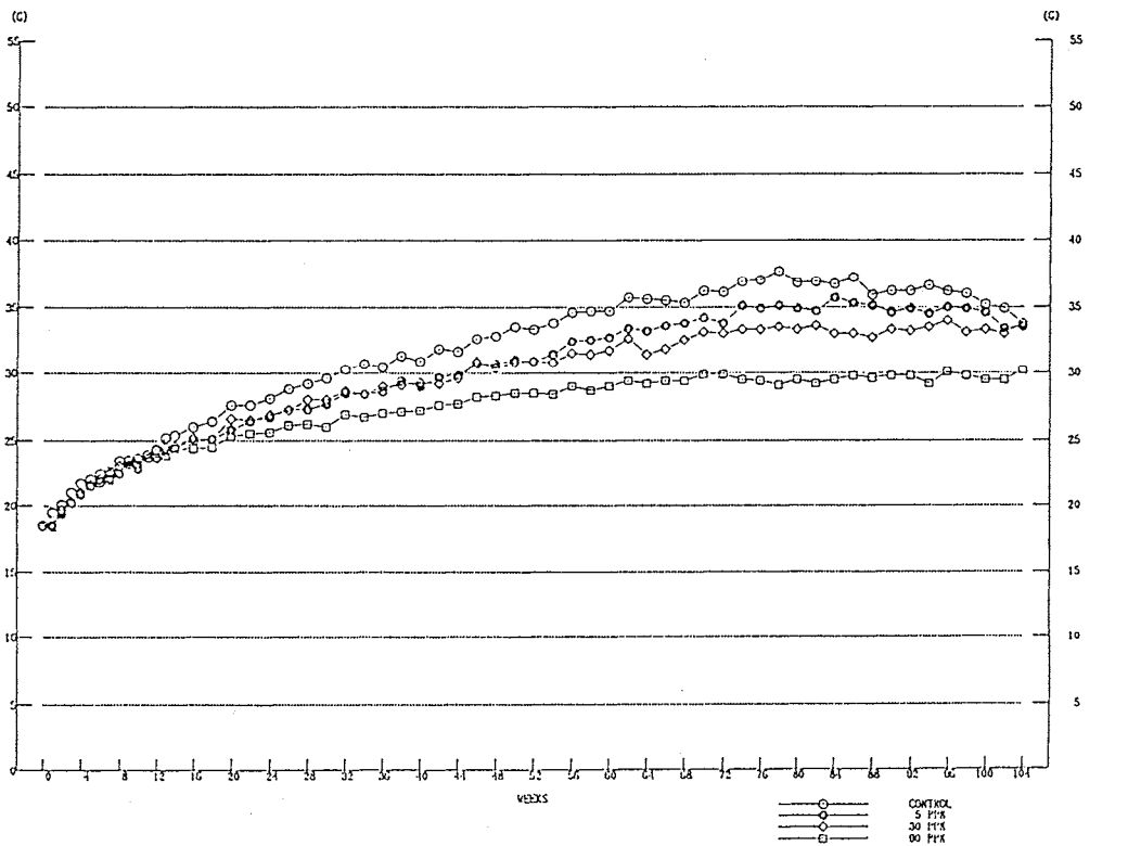
FIGURE 11 BODY WEIGHT CHANGES : MOUSE:FEMALE(TWO-YEAR STUDY)
