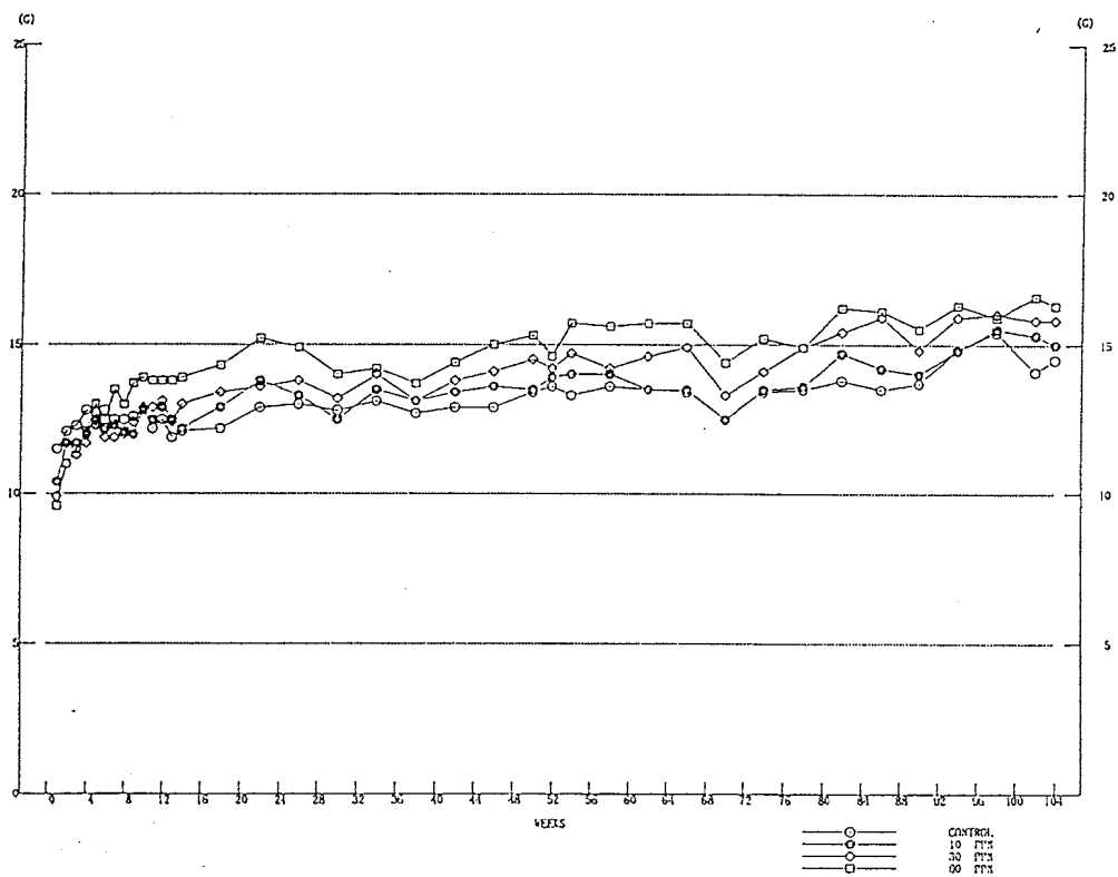
FIGURE 7 FOOD CONSUMPTION : RAT:FEMALE(TWO-YEAR STUDY)
