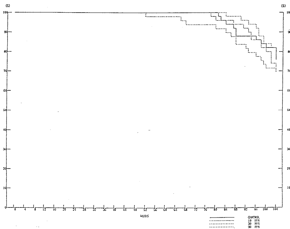
FIGURE 2 SURVIVAL ANIMAL RATE : RAT:MALE(TWO-YEAR STUDY)
