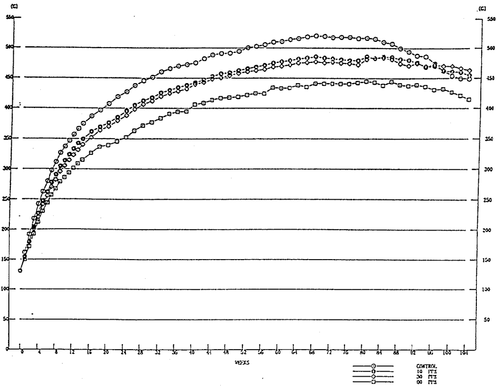
FIGURE 4 BODY WEIGHT CHANGES : RAT:MALE (TWO-YEAR STUDY)
