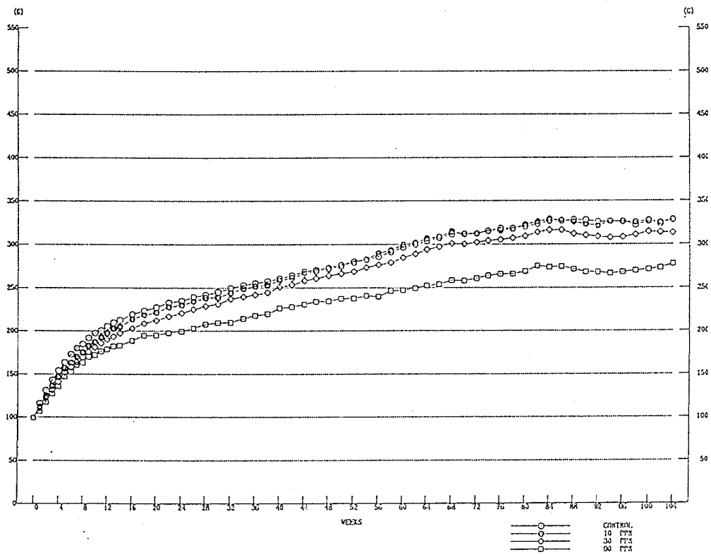
FIGURE 5 BODY WEIGHT CHANGES : RAT:FEMALE (TWO-YEAR STUDY)
