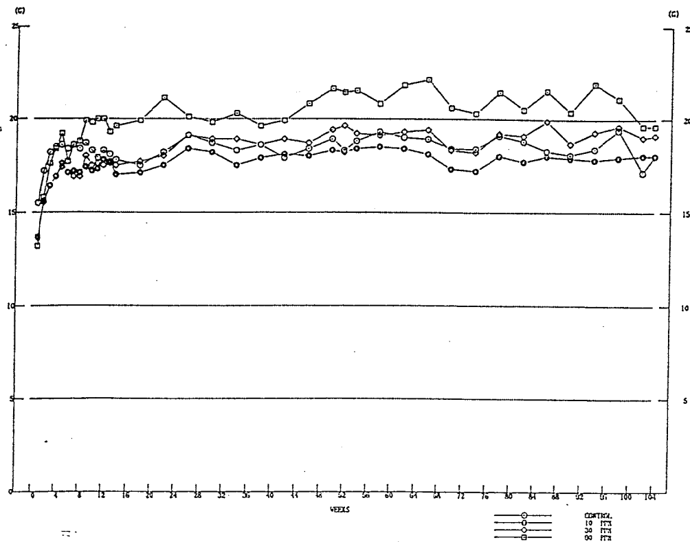
FIGURE 6 FOOD CONSUMPTION : RAT:MALE(TWO-YEAR STUDY)
