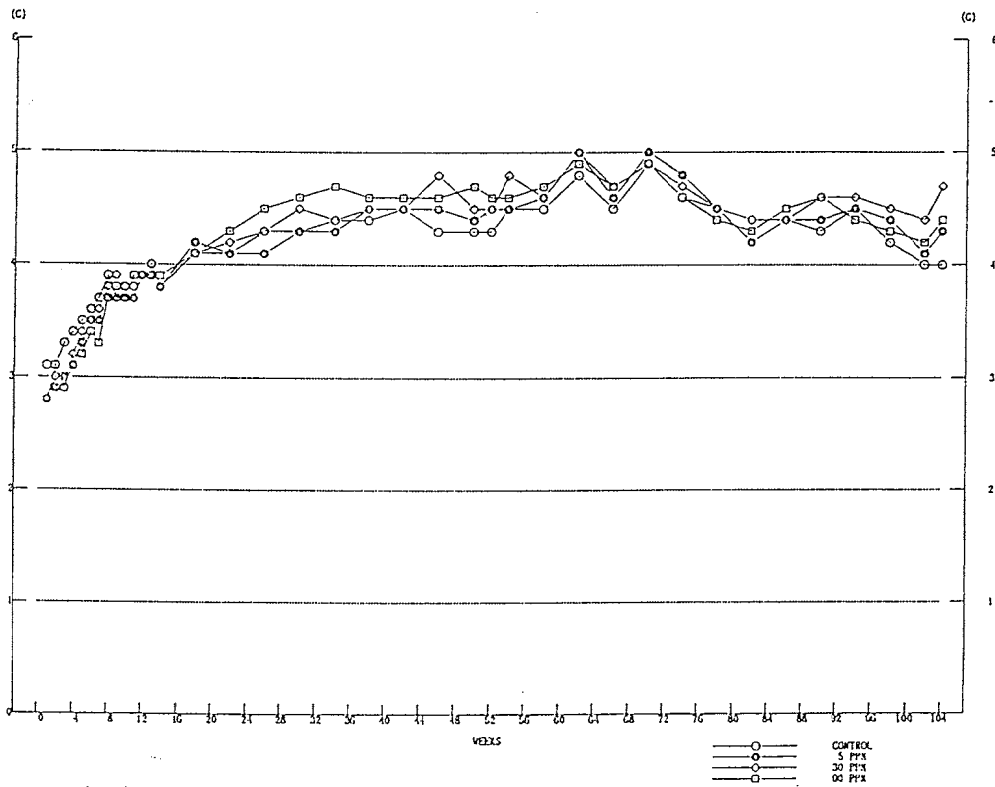
FIGURE 13 FOOD CONSUMPTION : MOUSE:FEMALE (TWO-YEAR STUDY)
