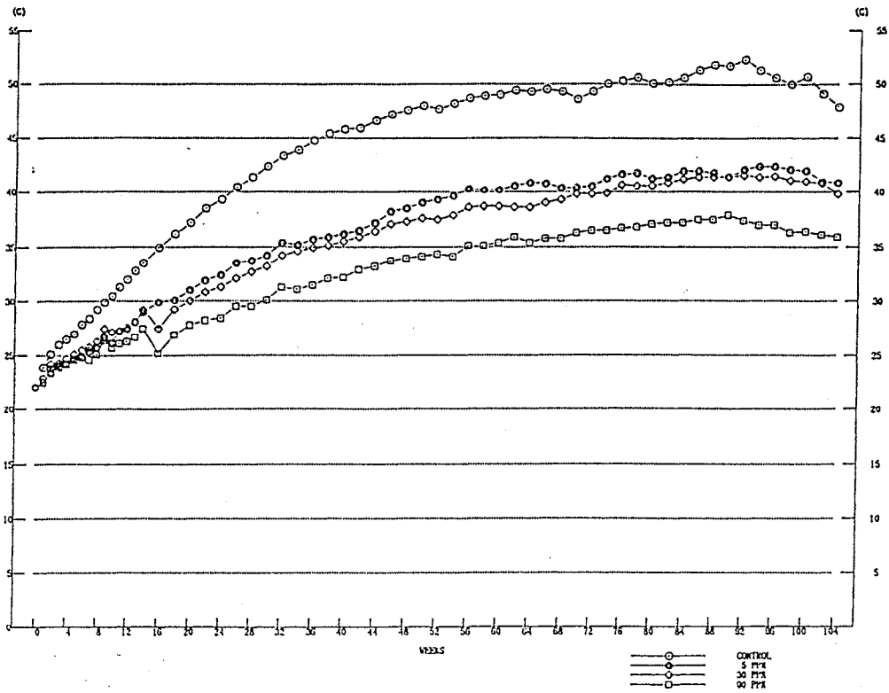
FIGURE 10 BODY WEIGHT CHANGES : MOUSE:MALE(TWO-YEAR STUDY)
