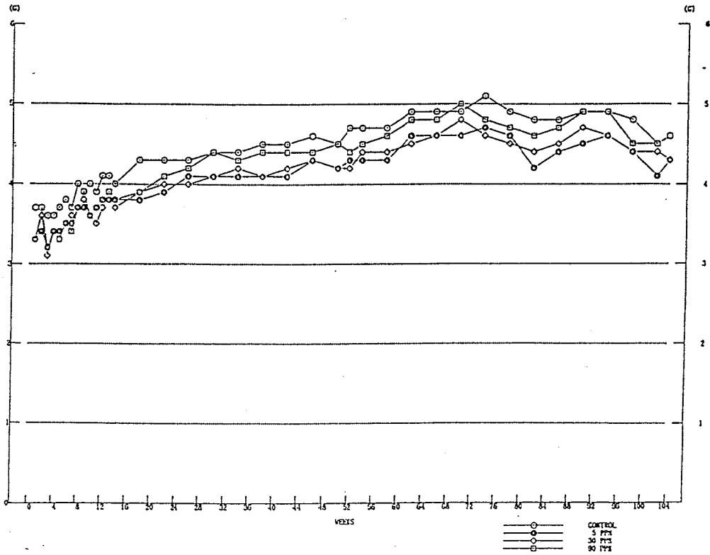
FIGURE 12 FOOD CONSUMPTION : MOUSE:MALE (TWO-YEAR STUDY)
