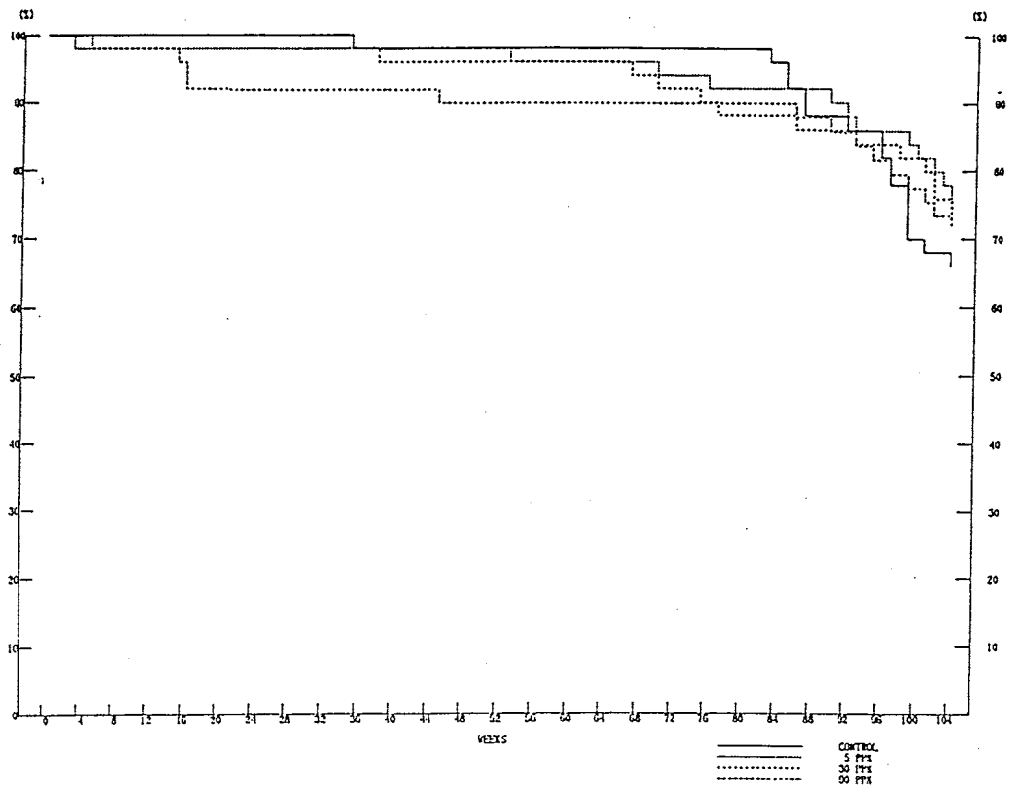
FIGURE 8 SURVIVAL ANIMAL RATE : MOUSE:MALE (TWO-YEAR STUDY)
