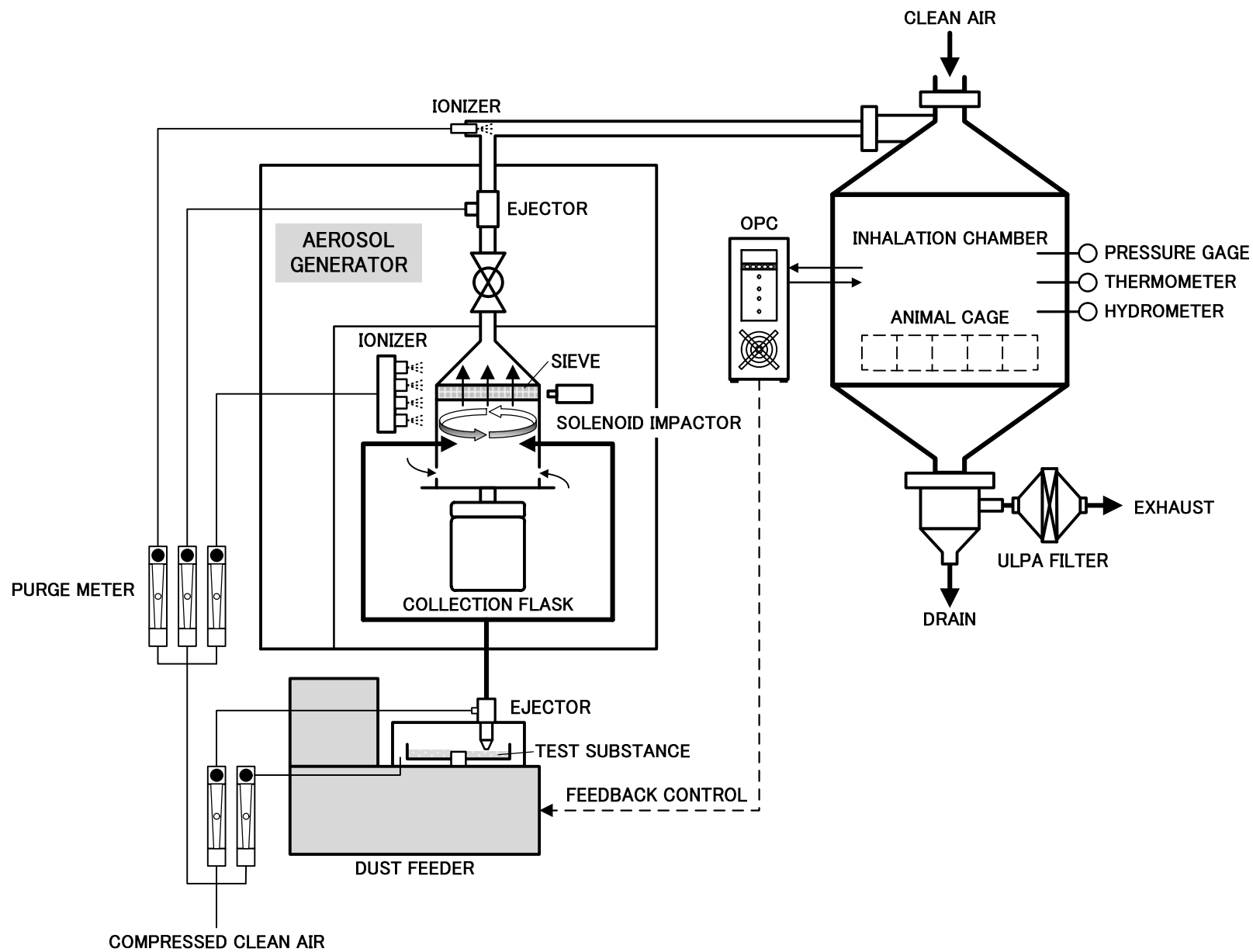
FIGURE 1 TITANIUM DIOXIDE AEROSOL GENERATION AND INHALATION EXPOSURE SYSTEM
