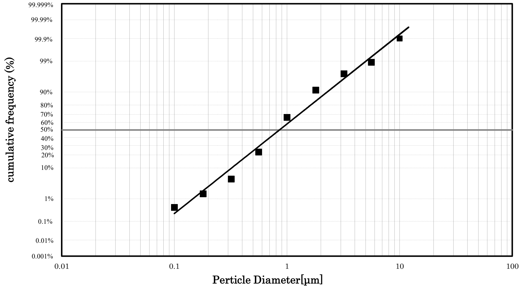
FIGURE 5 PARTICLE SIZE DISTRIBUTION CURVE 25 mg/m 3
