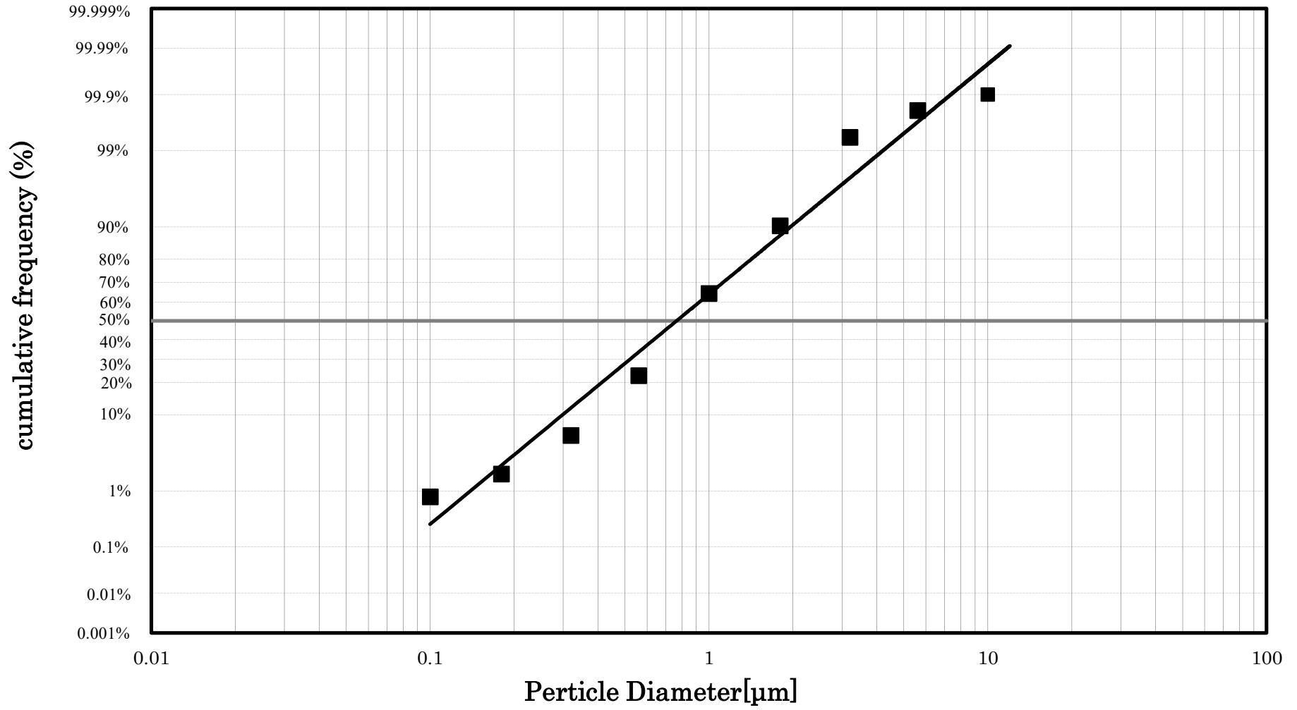
FIGURE 2 PARTICLE SIZE DISTRIBUTION CURVE 0.2 mg/m 3
