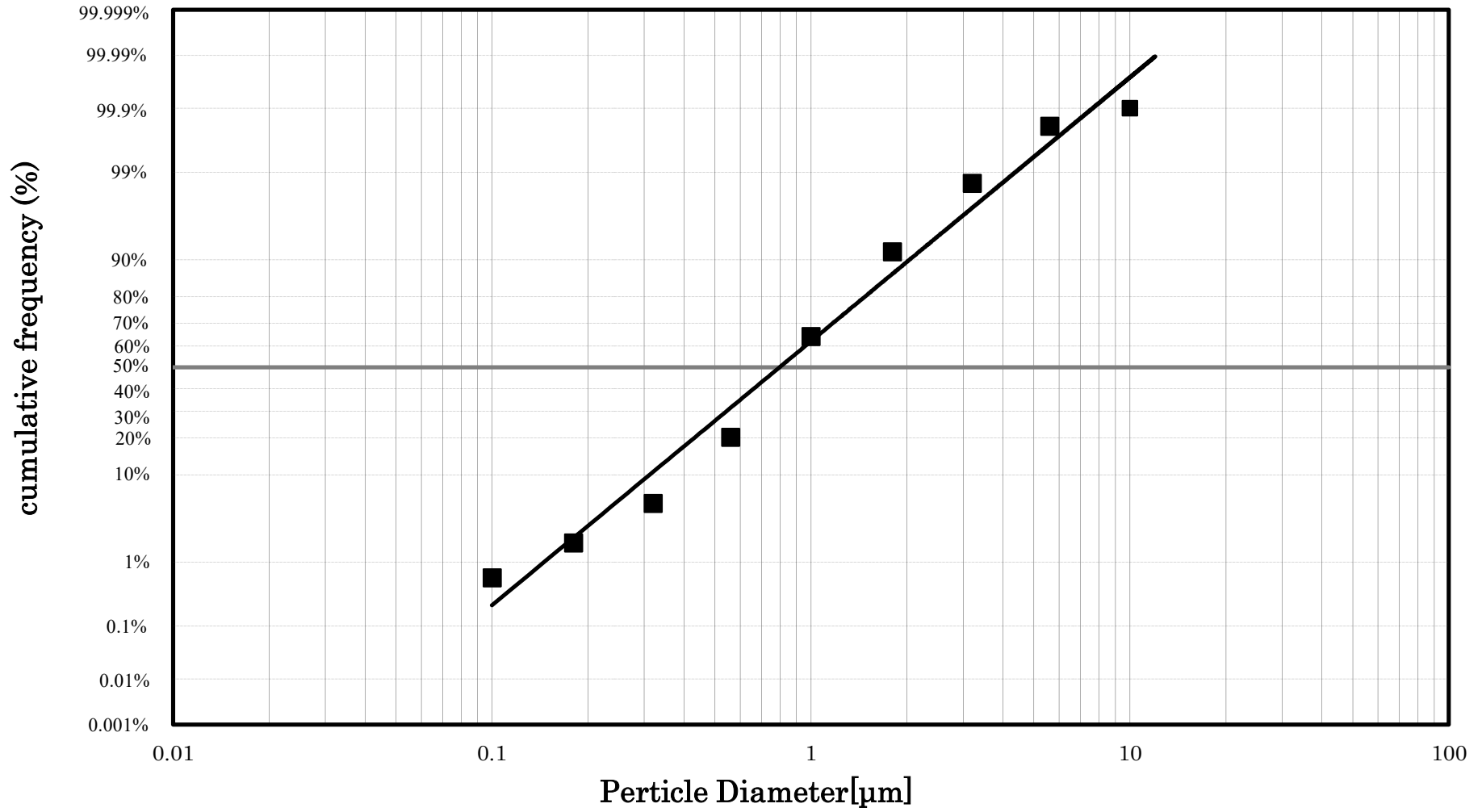
FIGURE 4 PARTICLE SIZE DISTRIBUTION CURVE 5 mg/m 3
