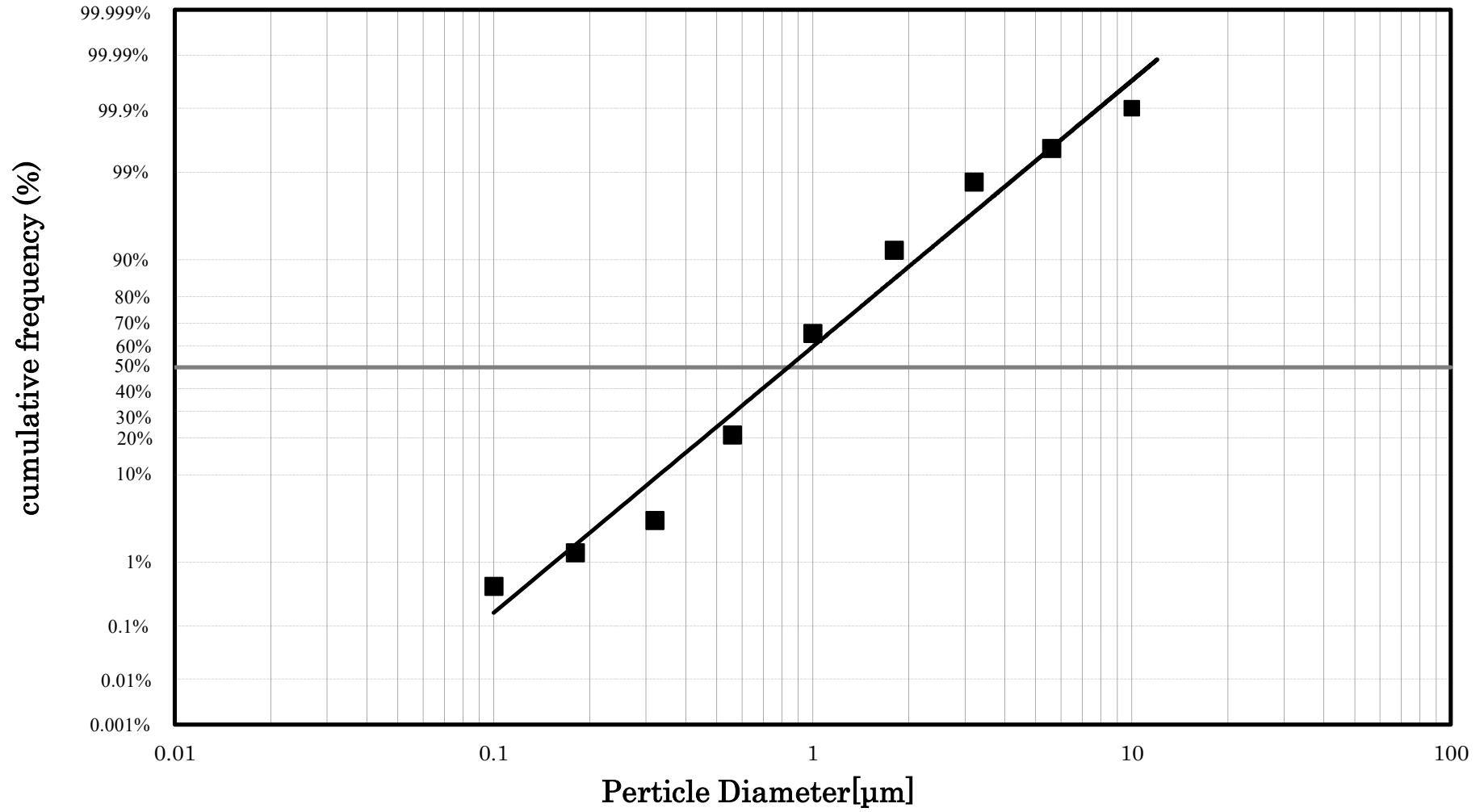
FIGURE 3 PARTICLE SIZE DISTRIBUTION CURVE 1 mg/m 3
