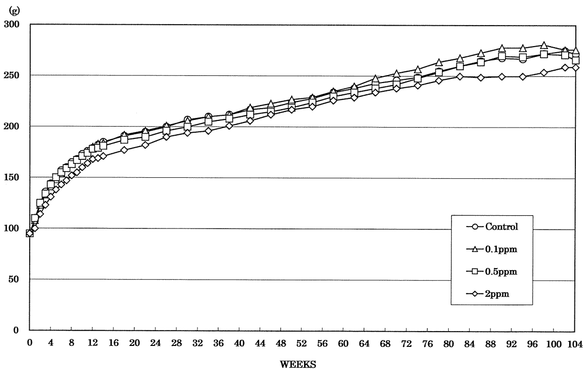
FIGURE 4 BODY WEIGHT CHANGES OF FEMALE RATS IN THE 2-YEAR INHALATION STUDY OF ACROLEIN
