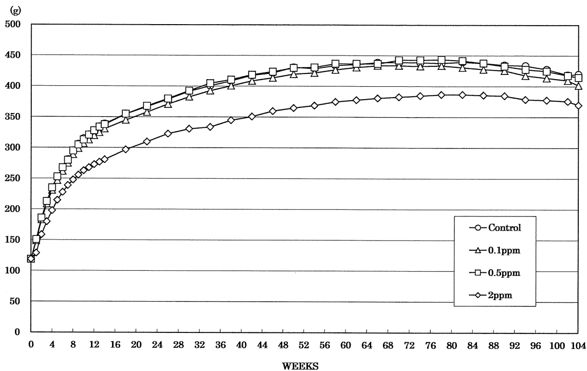
FIGURE 3 BODY WEIGHT CHANGES OF MALE RATS IN THE 2-YEAR INHALATION STUDY OF ACROLEIN
