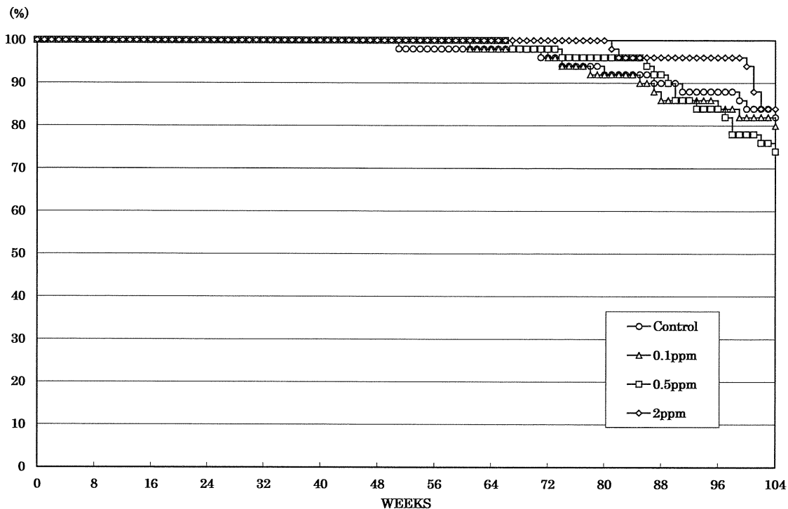
FIGURE 1 SURVIVAL ANIMAL RATE OF MALE RATS IN THE 2-YEAR INHALATION STUDY OF ACROLEIN
