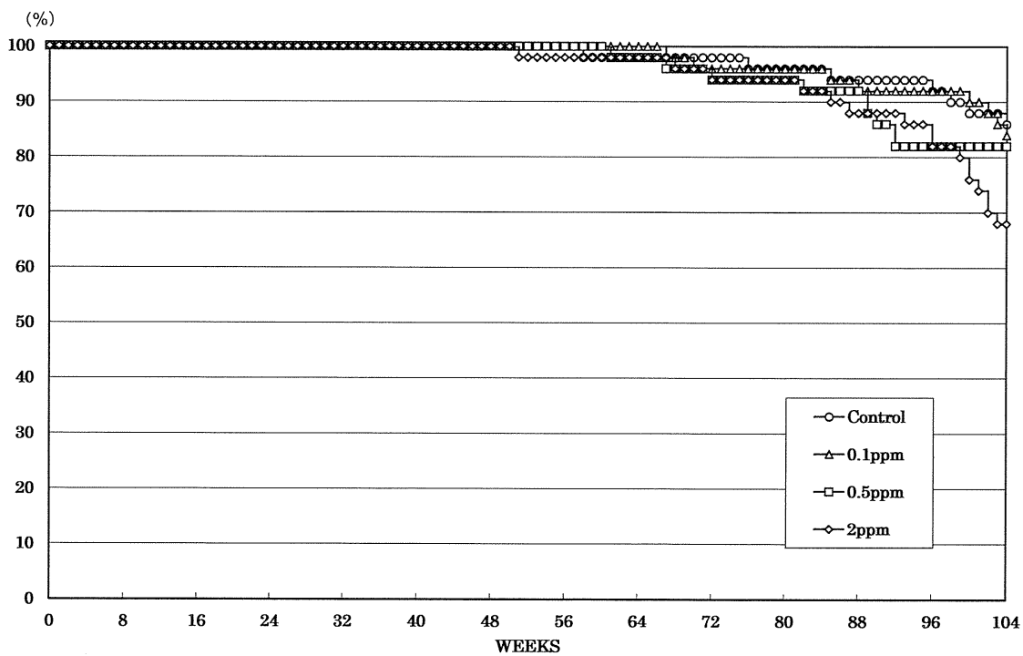
FIGURE 2 SURVIVAL ANIMAL RATE OF FEMALE RATS IN THE 2-YEAR INHALATION STUDY OF ACROLEIN
