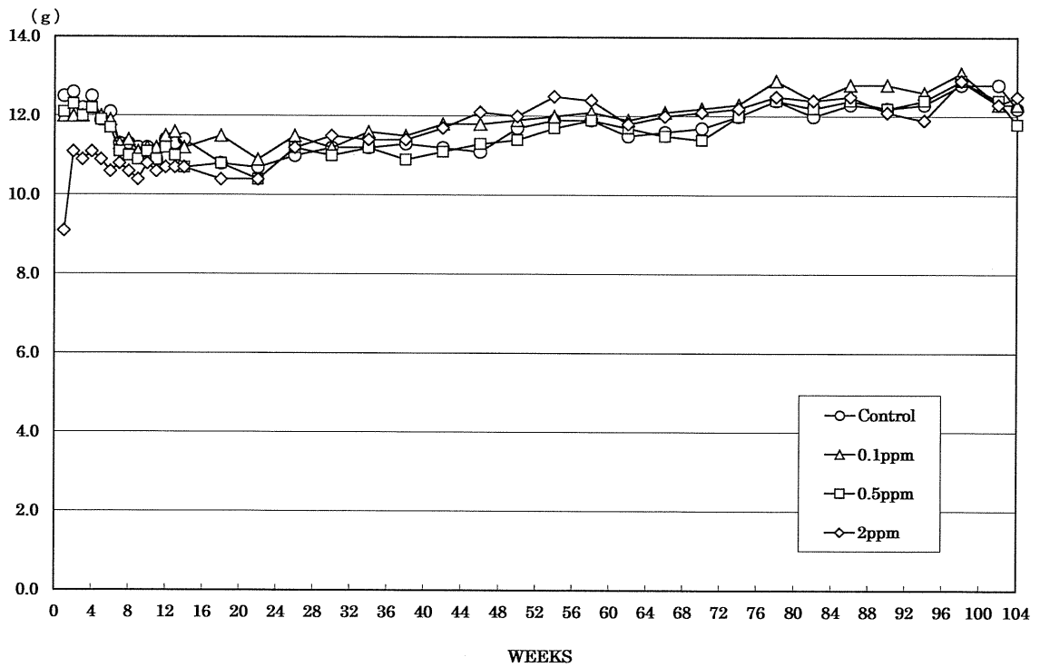
FIGURE 6 FOOD CONSUMPTION CHANGES OF FEMALE RATS IN THE 2-YEAR INHALATION STUDY OF ACROLEIN
