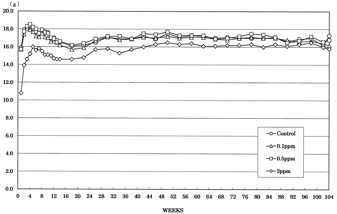
FIGURE 5 FOOD CONSUMPTION CHANGES OF MALE RATS IN THE 2-YEAR INHALATION STUDY OF ACROLEIN
