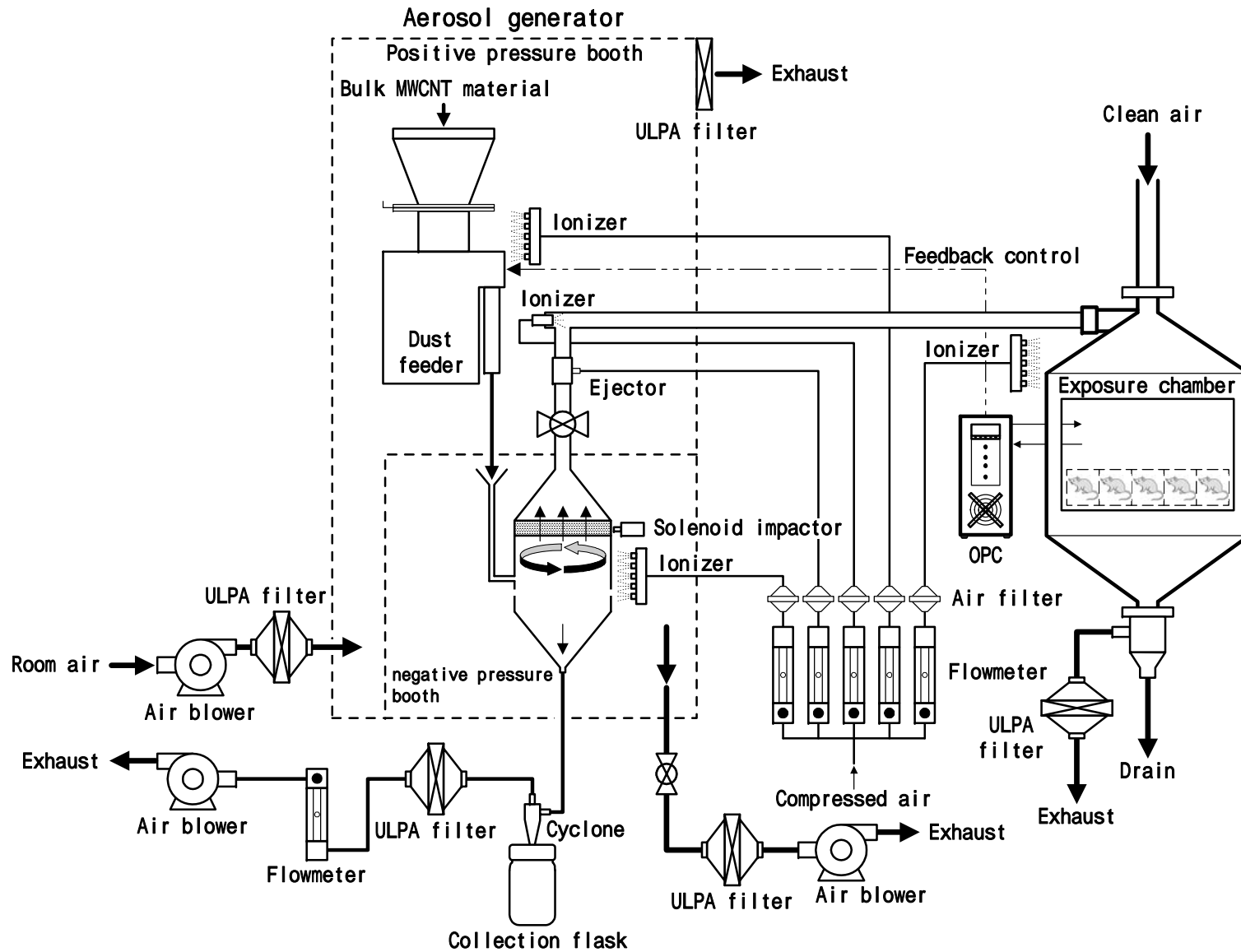
FIGURE 1 MWCNT AEROSOL GENERATION AND INHALATION EXPOSURE SYSTEM
