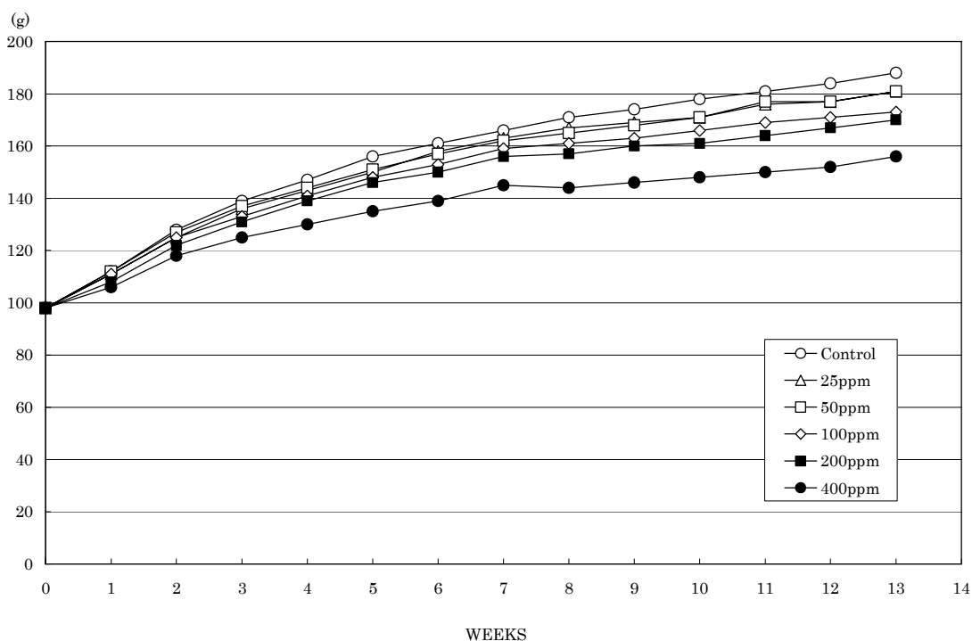
FIGURE 3 BODY WEIGHT CHANGES OF FEMALE RATS IN THE 13-WEEK INHALATION STUDY OF ETHYLENE GLYCOL MONOETHYL ETHER ACETATE
