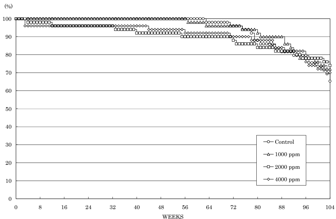
FIGURE 2 SURVIVAL ANIMAL RATE OF MALE MICE IN THE 2-YEAR INHALATION STUDY OF ISOPROPYL ACETATE
