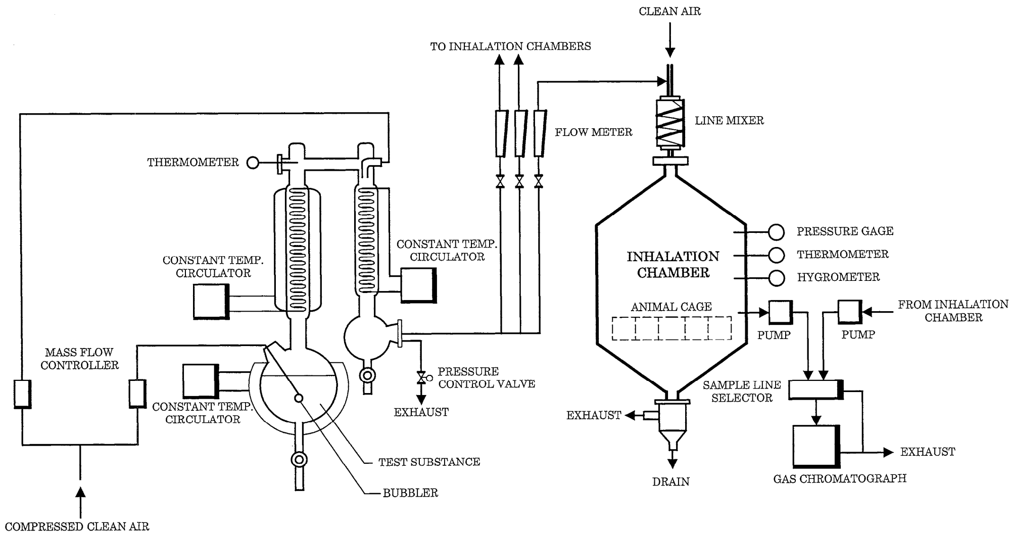
FIGURE 1 PROPIONITRILE VAPOR GENERATION SYSTEM AND INHALATION SYSTEM
