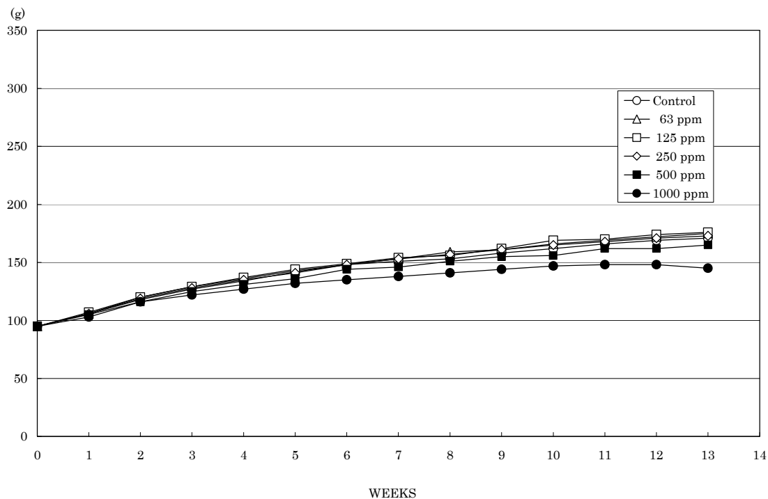
FIGURE 3 BODY WEIGHT CHANGES OF FEMALE RATS IN THE 13-WEEK INHALATION STUDY OF 1-BROMOBUTANE
