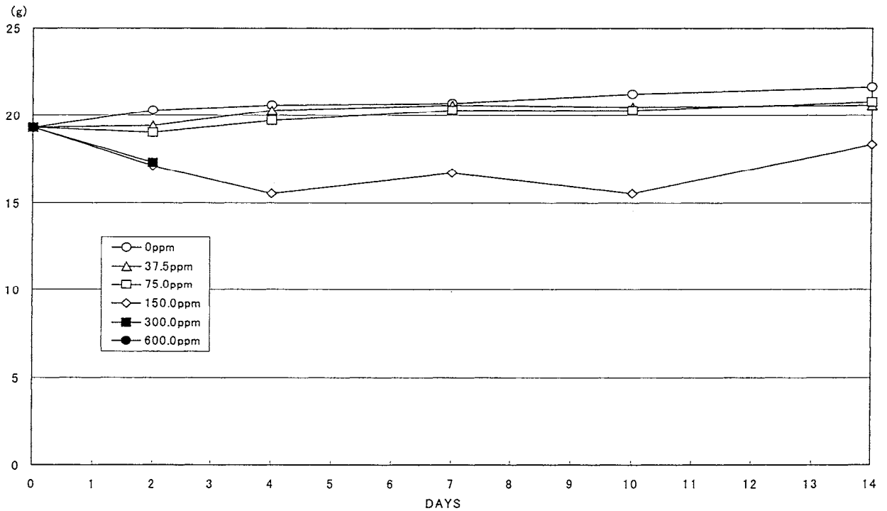
FIGURE 3 BODY WEIGHT CHANGES OF FEMALE MICE IN THE 2-WEEK INHALATION STUDY OF GLYCIDOL
