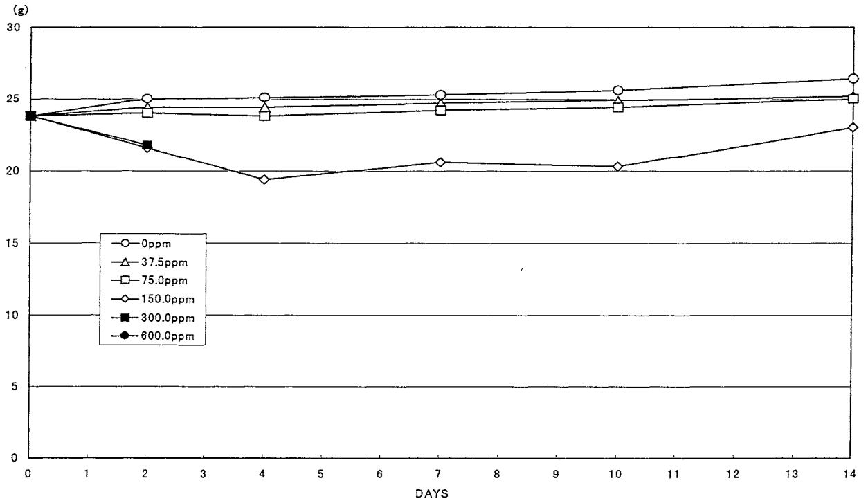
FIGURE 2 BODY WEIGHT CHANGES OF MALE MICE IN THE 2-WEEK INHALATION STUDY OF GLYCIDOL
