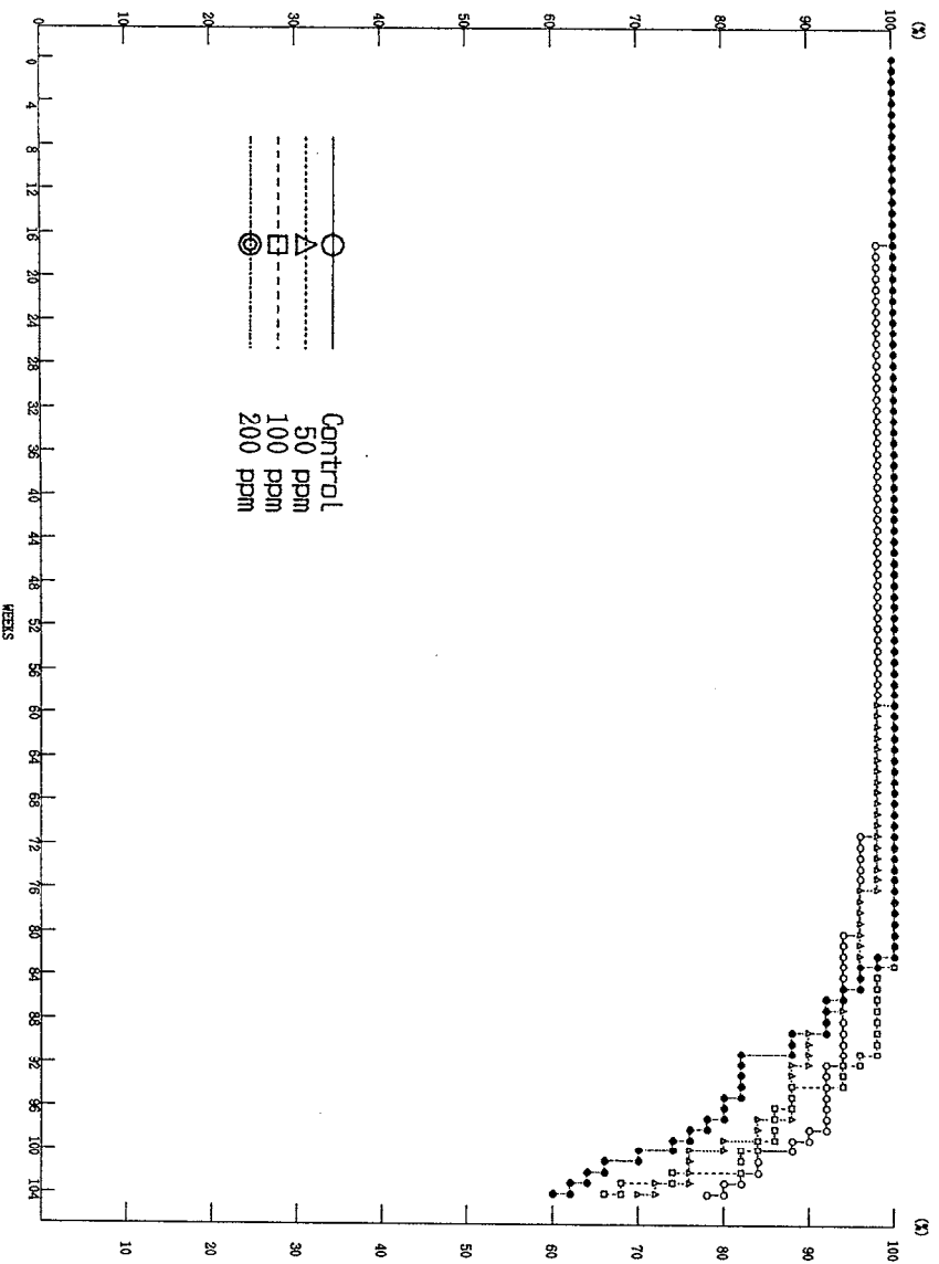
FIGURE 2 SURVIVAL ANIMAL RATE OF MALE RATS IN THE 2-YEAR INHALATION STUDY OF 2-METHALLYL CHLORIDE
