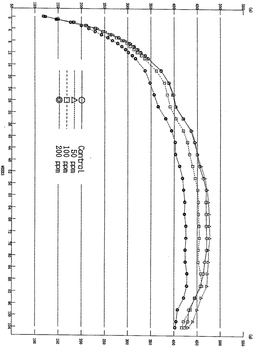
FIGURE 4 BODY WEIGHT CHANGES OF MALE RATS IN THE 2-YEAR INHALATION STUDY OF 2-METHALLYL CHLORIDE
