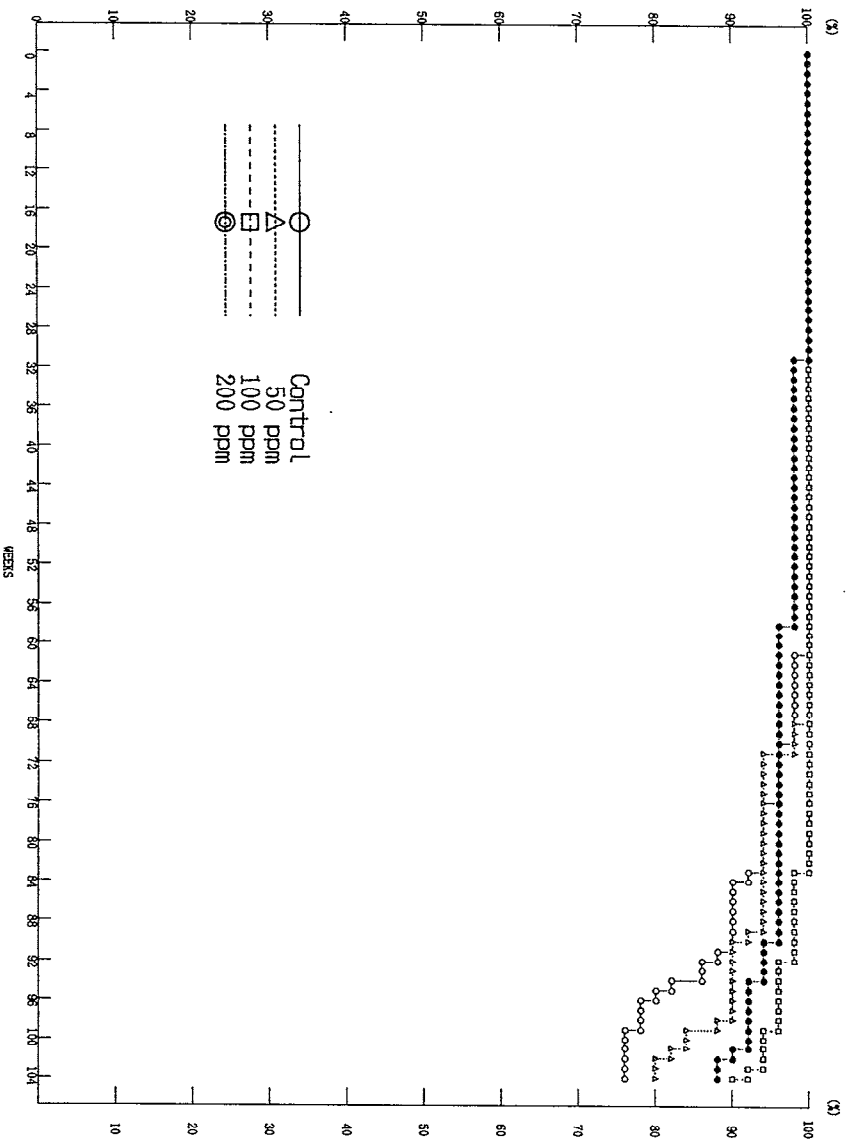
FIGURE 3 SURVIVAL ANIMAL RATE OF FEMALE RATS IN THE 2-YEAR INHALATION STUDY OF 2-METHALLYL CHLORIDE
