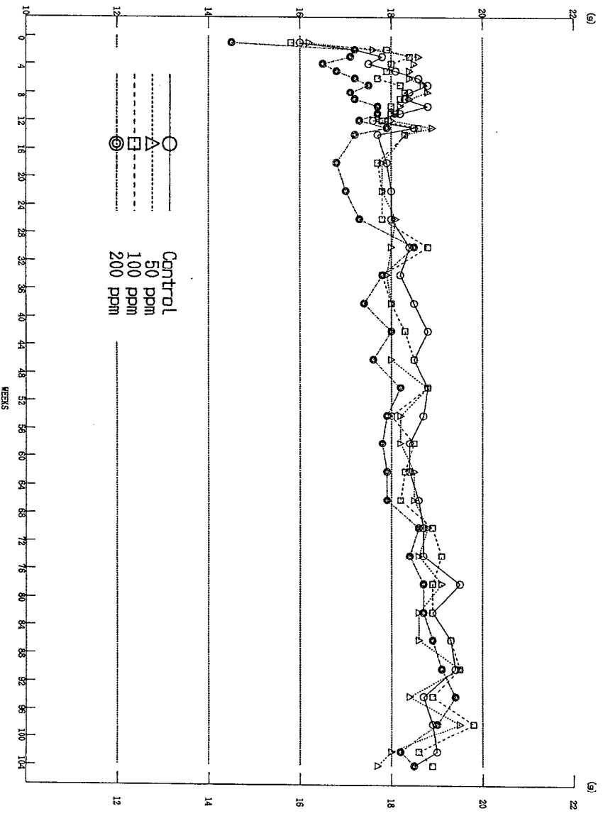
FIGURE 6 FOOD CONSUMPTION CHANGES OF MALE RATS IN THE 2-YEAR INHALATION STUDY OF 2-METHALLYL CHLORIDE
